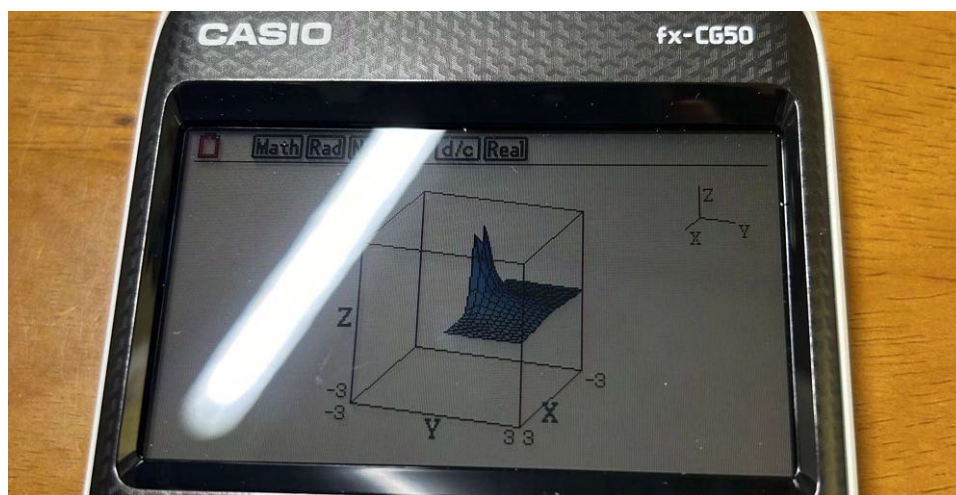
The Graph of E.
